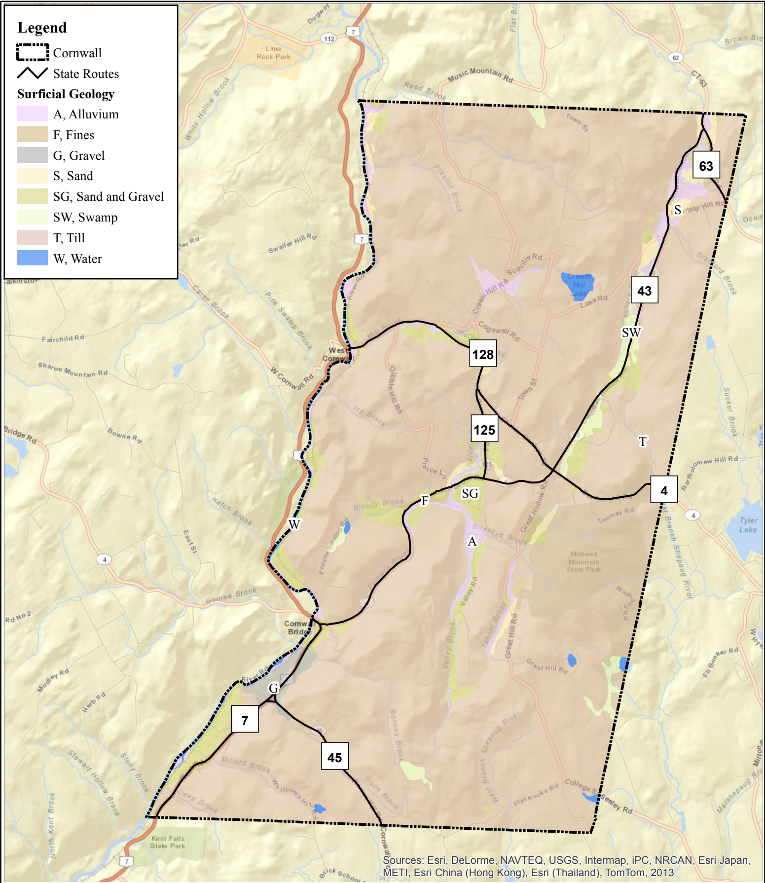
Figure 2-4: Surficial Geology
